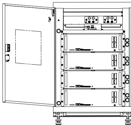
Internal drawing
