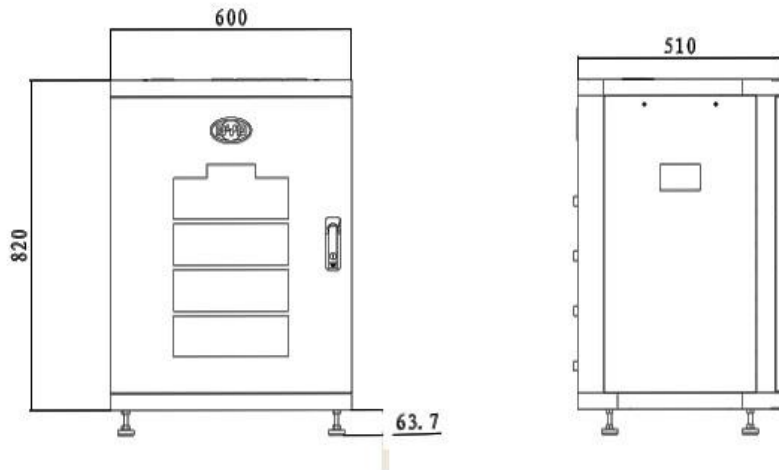
Structure dimension drawing
